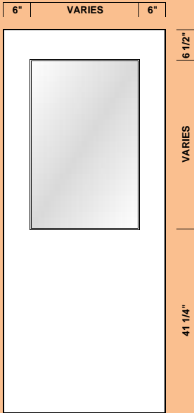
VL6 - HALF LITE
