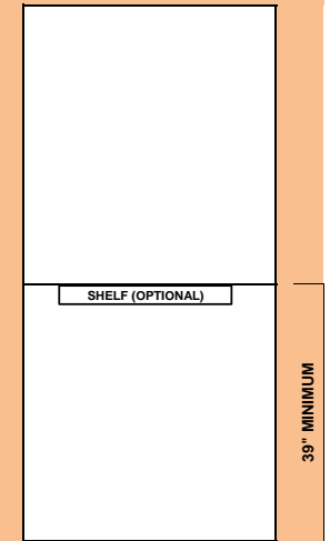
DUTCH DOOR
