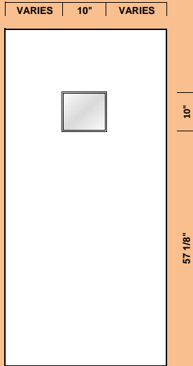
VL1 - 10" x 10"
